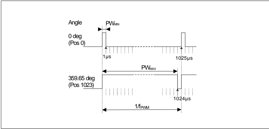
Figure 28: PWM Output Signal
