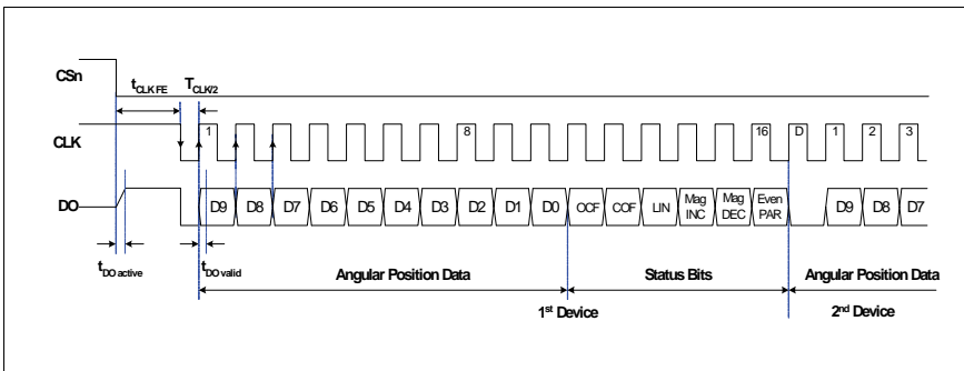
Figure 25: Daisy Chain Mode Data Transfer
