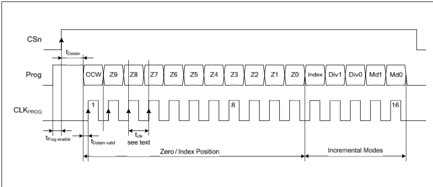
Figure 33: Programming Access – Write Data (section of Figure 34)
