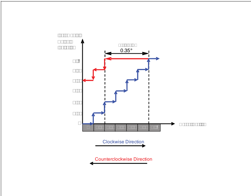
Figure 27: Hysteresis Window for Incremental Outputs
