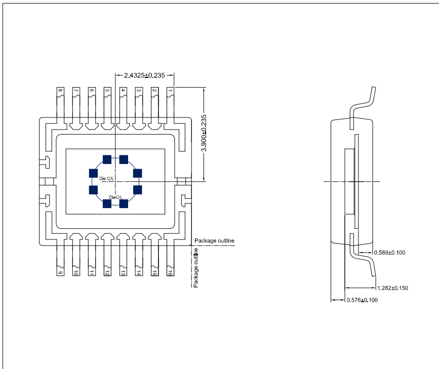
Figure 47: Hall Element Positions
