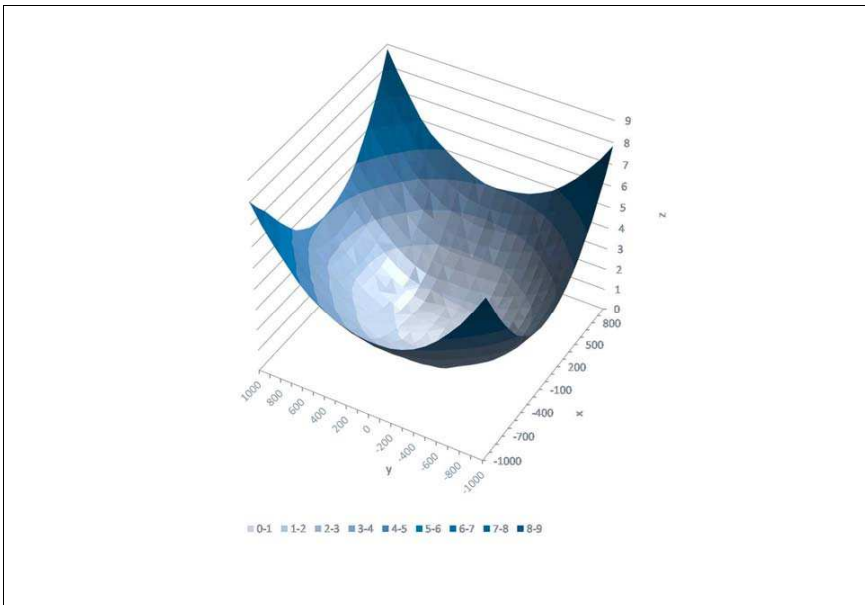
Figure 44: Example of Linearity Error Over XY Misalignment
