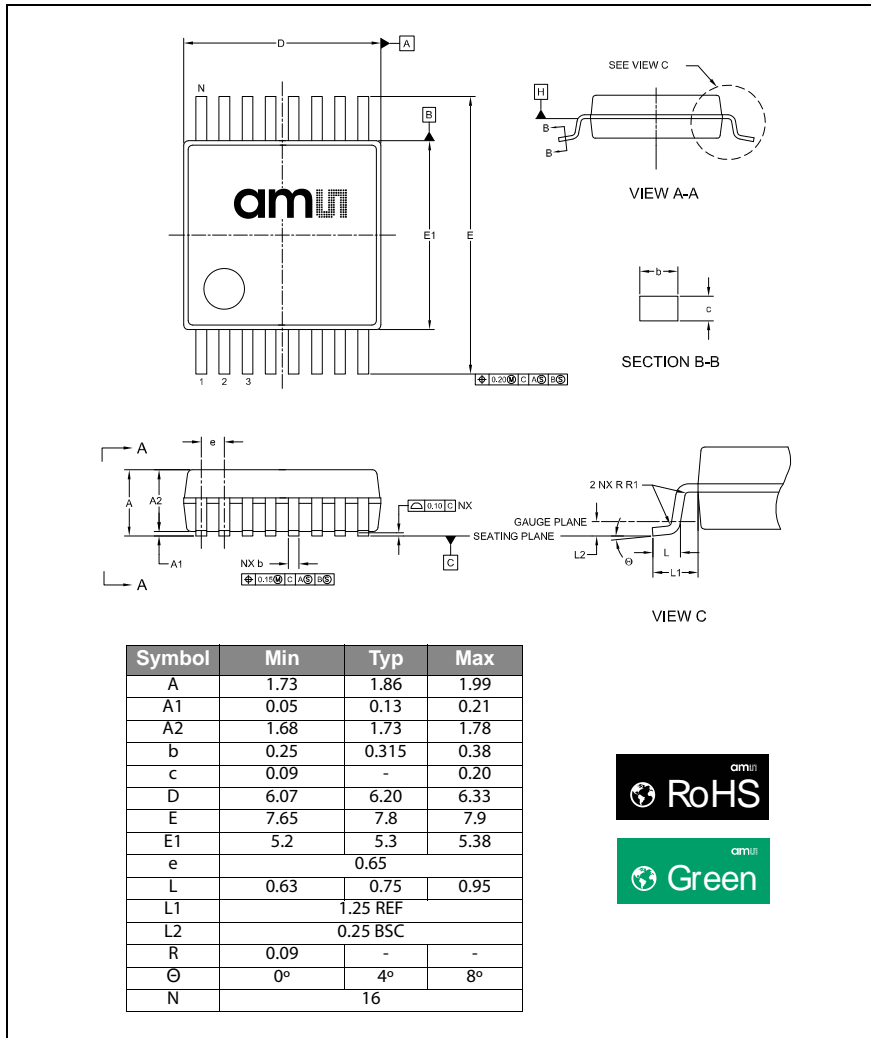
Figure 48: 16-Lead Shrink Small Outline Package SSOP-16
