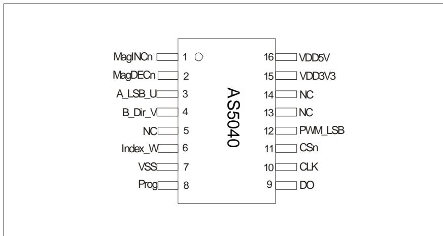
Figure 4: Pin Configuration SSOP16
