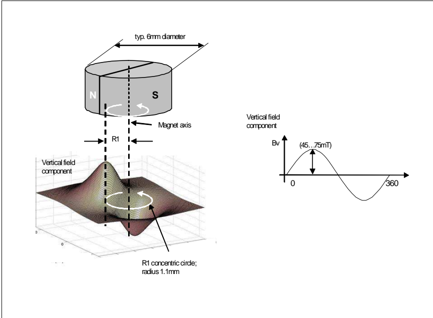
Figure 40: Typical Magnet and Magnetic Field Distribution
