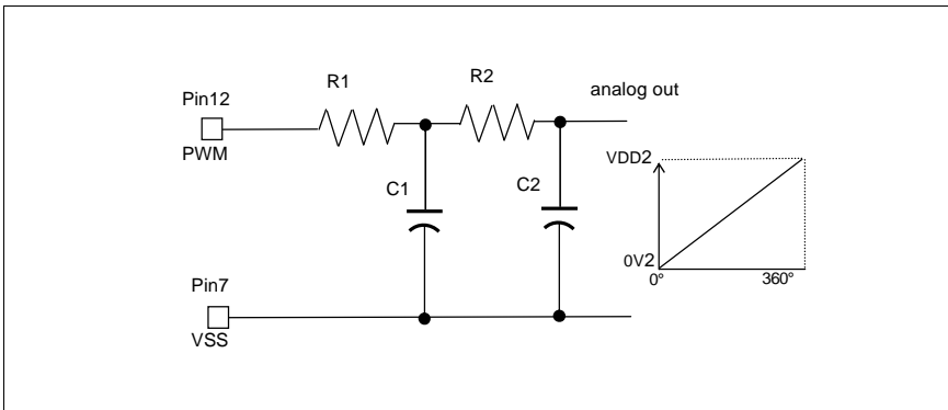
Simple Passive 2 nd Order RC Low Pass Filter
