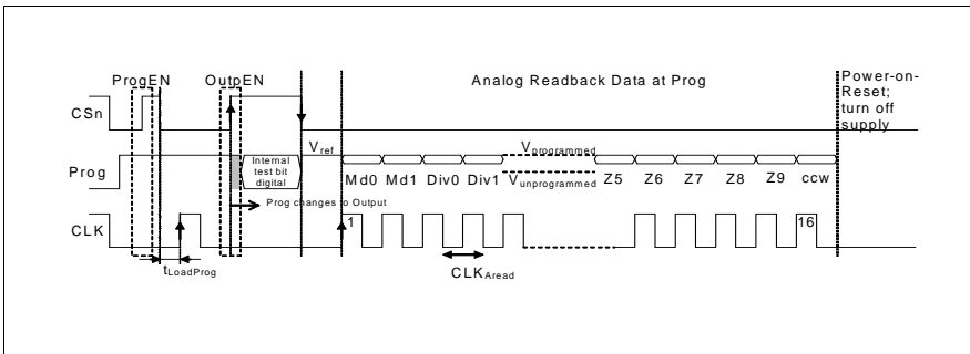
Figure 37: OTP Register Analog Read
