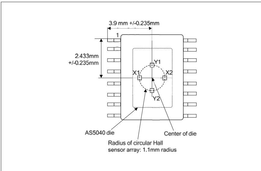
Figure 43: Arrangement of Hall Sensor Array on Chip (principle)
