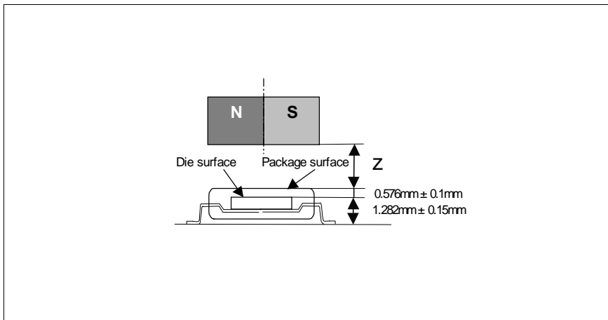
Figure 42: Vertical Placement of the Magnet
