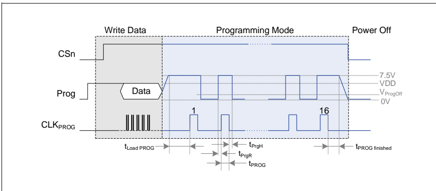
Figure 34: Complete Programming Sequence
