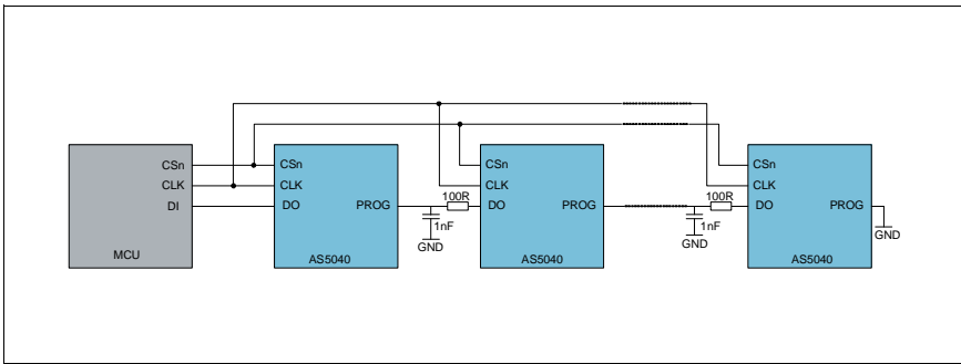
Figure 24: Daisy Chain Hardware Configuration
