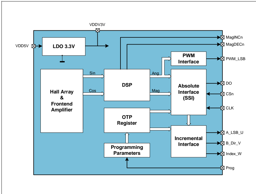
Figure 3: AS5040 Block Diagram
