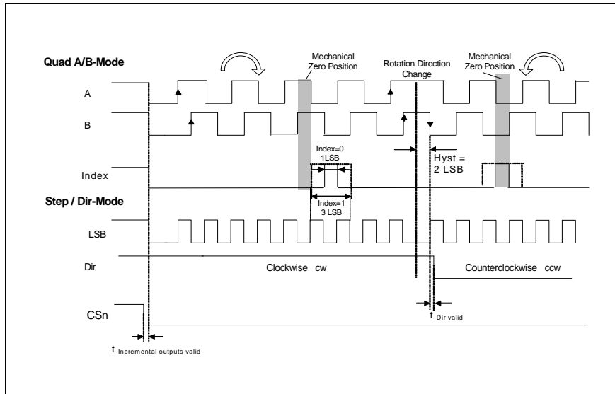
Figure 26: Incremental Output Modes
