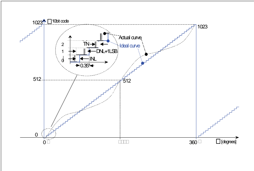
Figure 16: Integral and Differential Non-Linearity Example (Exaggerated Curve)
