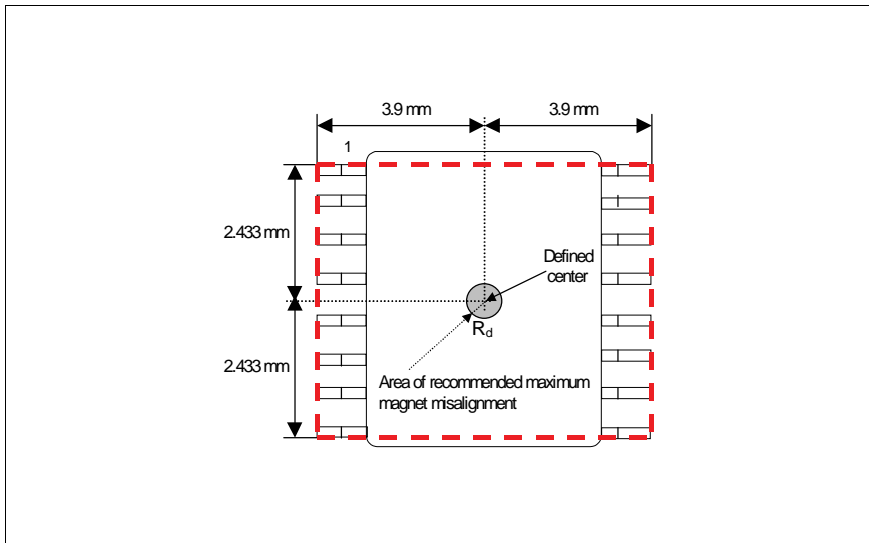
Figure 41: Defined IC Center and Magnet Displacement Radius
