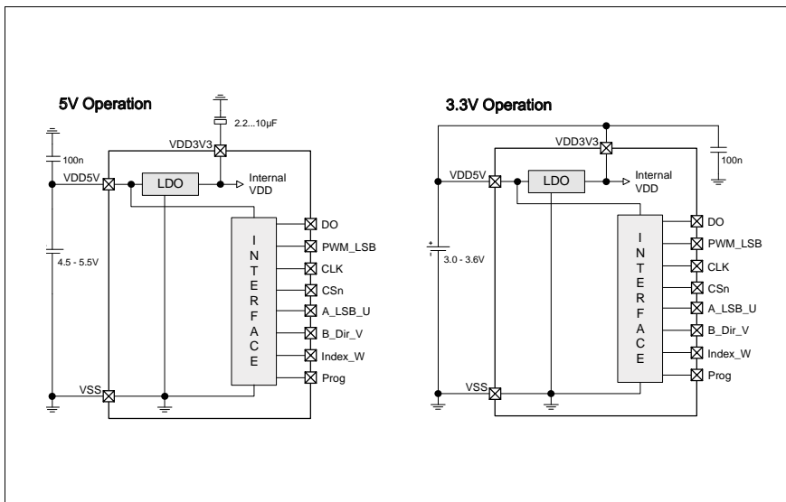
Figure 39: Connections for 5V / 3.3V Supply Voltages
