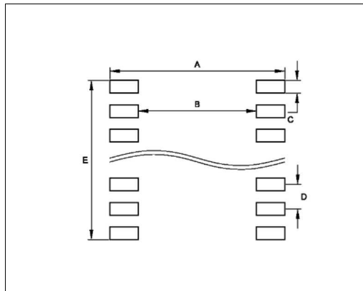
Figure 52: Recommended Footprint Data
