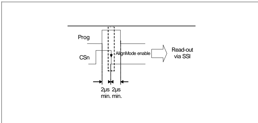
Figure 38: Enabling the Alignment Mode
