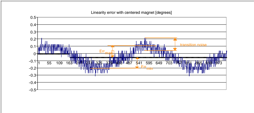
Figure 45: Example of Linearity Error Over 360°
