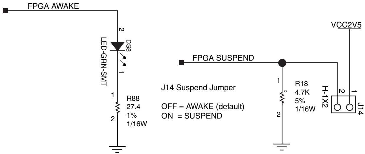
Figure 1-19: FPGA Awake LED and Suspend Jumper
