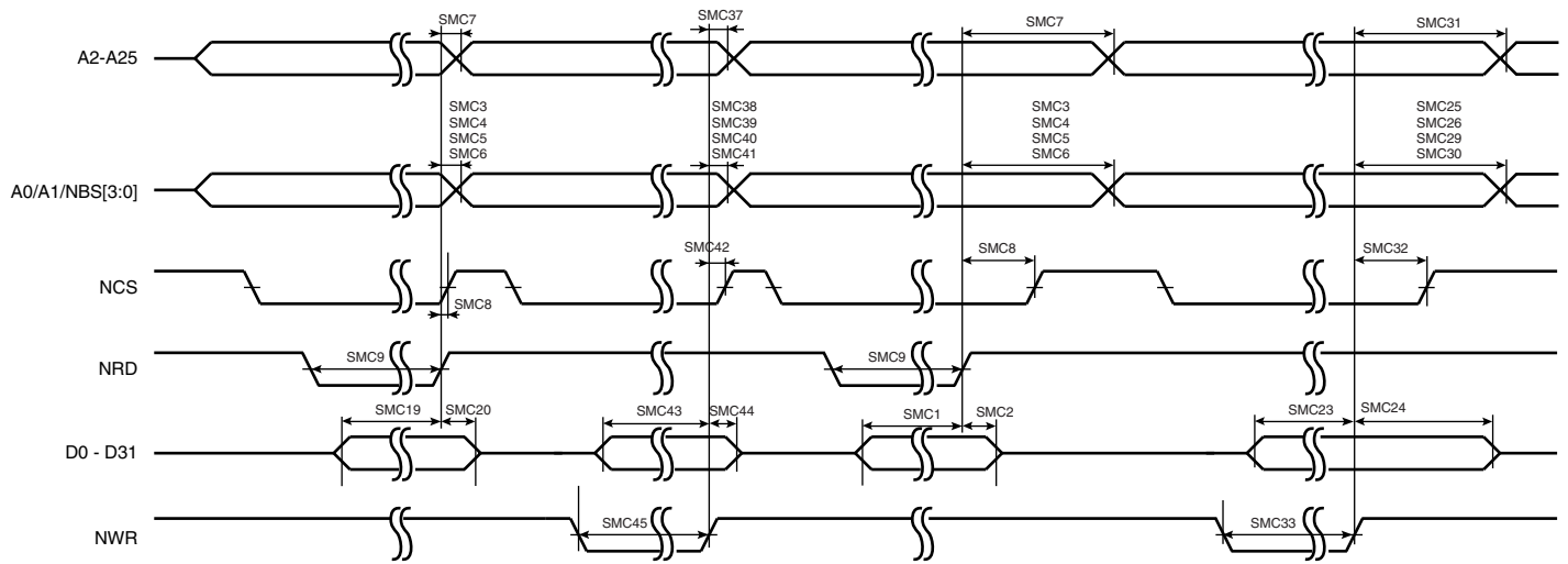
Figure 39-4. SMC Signals for NRD and NWR Controlled Access
