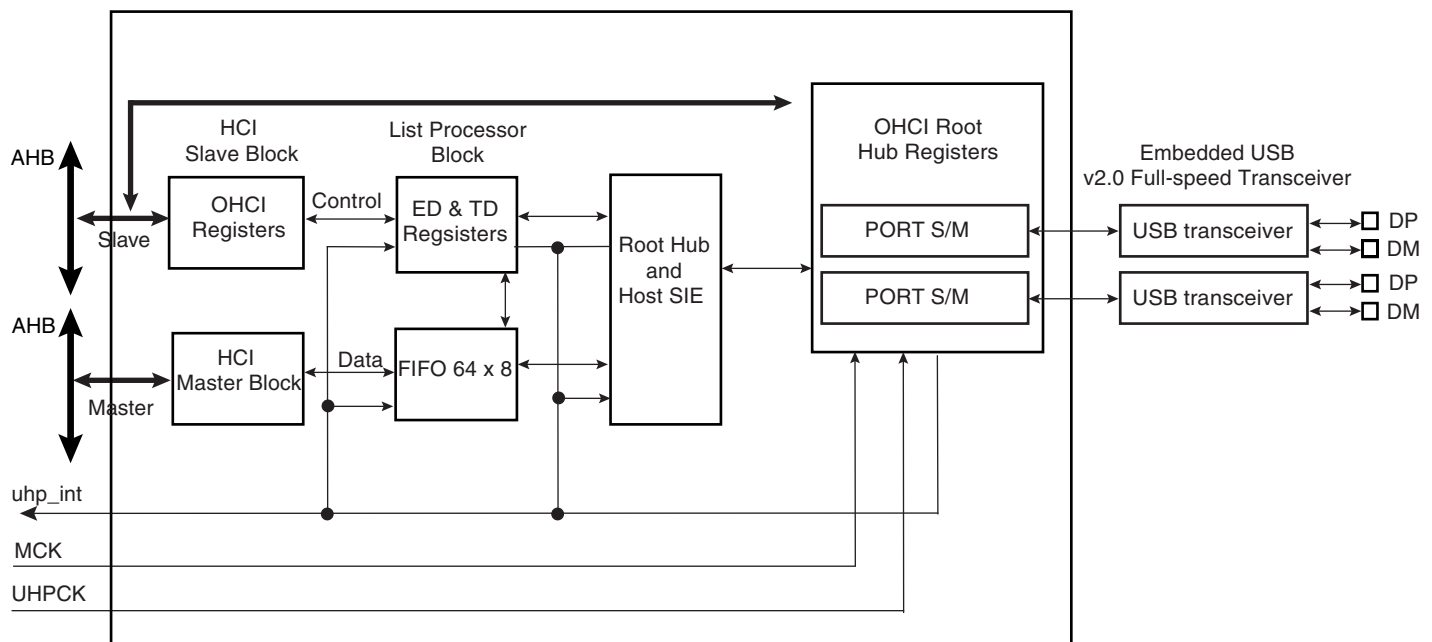
Figure 36-1. Block Diagram
