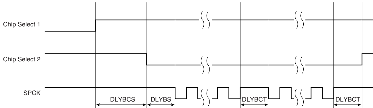
Figure 30-7. Programmable Delays
