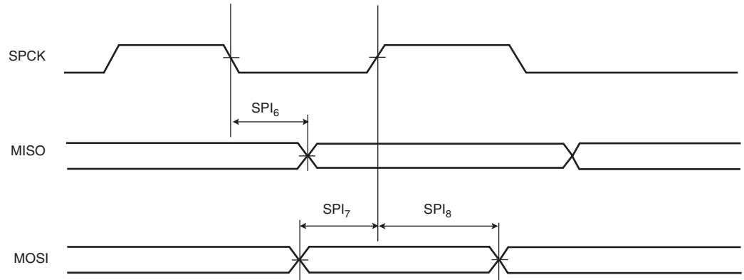
Figure 39-8. SPI Slave mode with (CPOL=0 and NCPHA=1) or (CPOL=1 and NCPHA=0)
