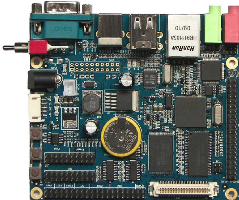
Embest SBC6000X Single Board Computer
