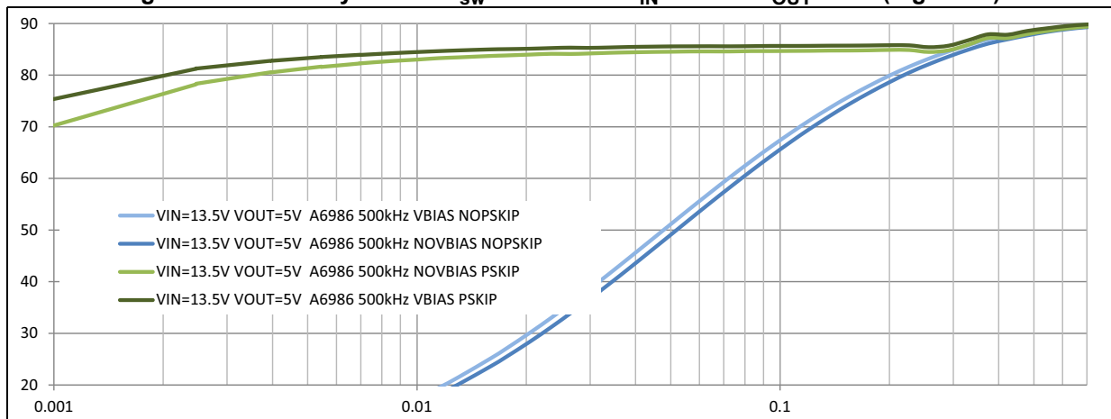
Figure 51. Efficiency curves: f_{sw} = 500 \text{ kHz} - V_{IN} = 13.5 \text{ V} - V_{OUT} = 5 \text{ V} (log scale)
