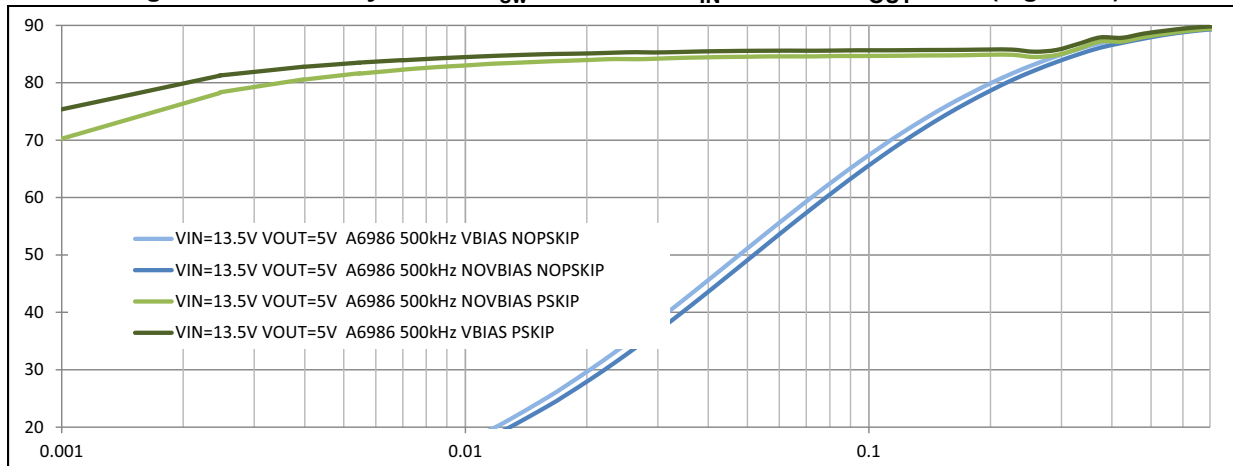
Figure 48. Efficiency curves: f_{sw} = 500 \text{ kHz} - V_{IN} = 24 \text{ V} - V_{OUT} = 3.3 \text{ V}
