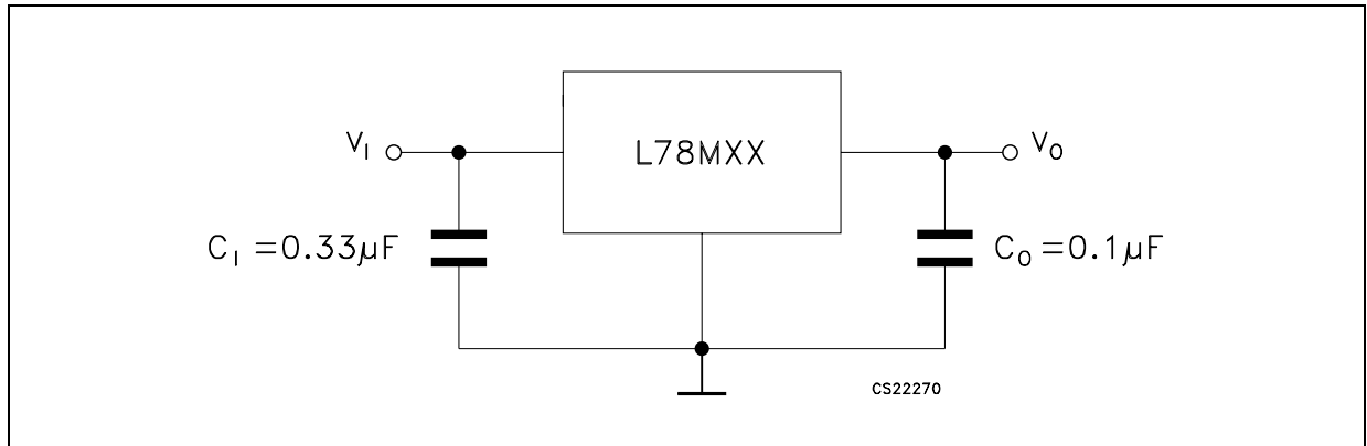
Figure 4. Application circuit
