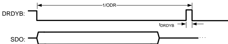
Figure 48. DRDYB Behavior
