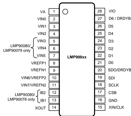
Figure 2. 28-pin HTSSOP
