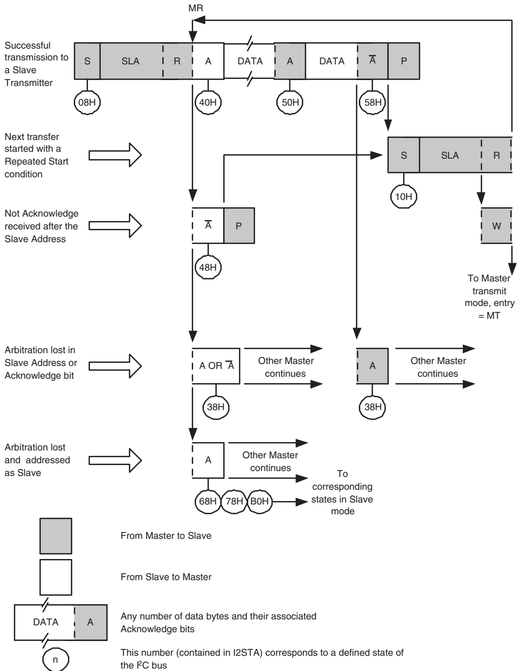
Fig 33. Format and states in the Master Receiver mode
