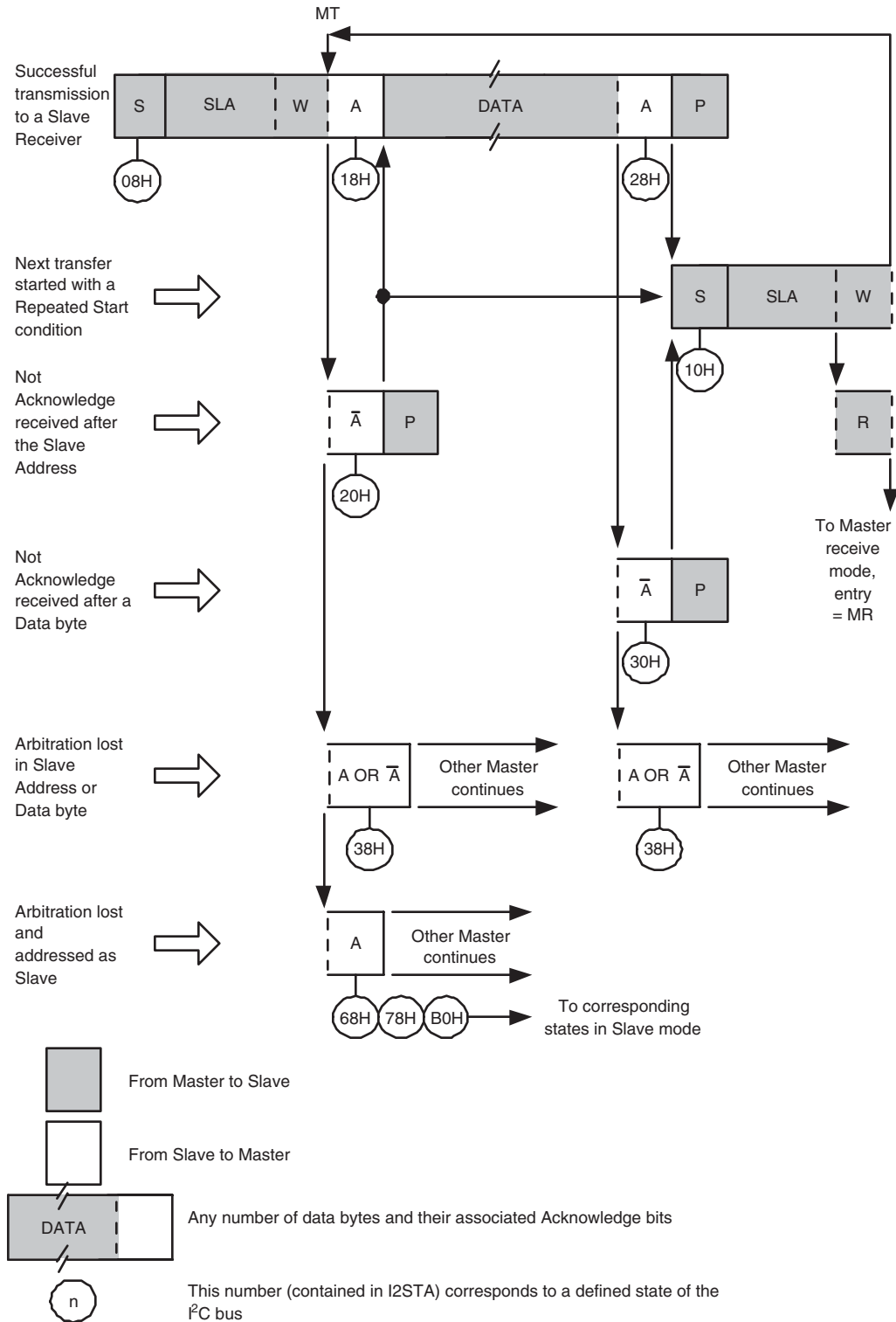
Fig 32. Format and states in the Master Transmitter mode
