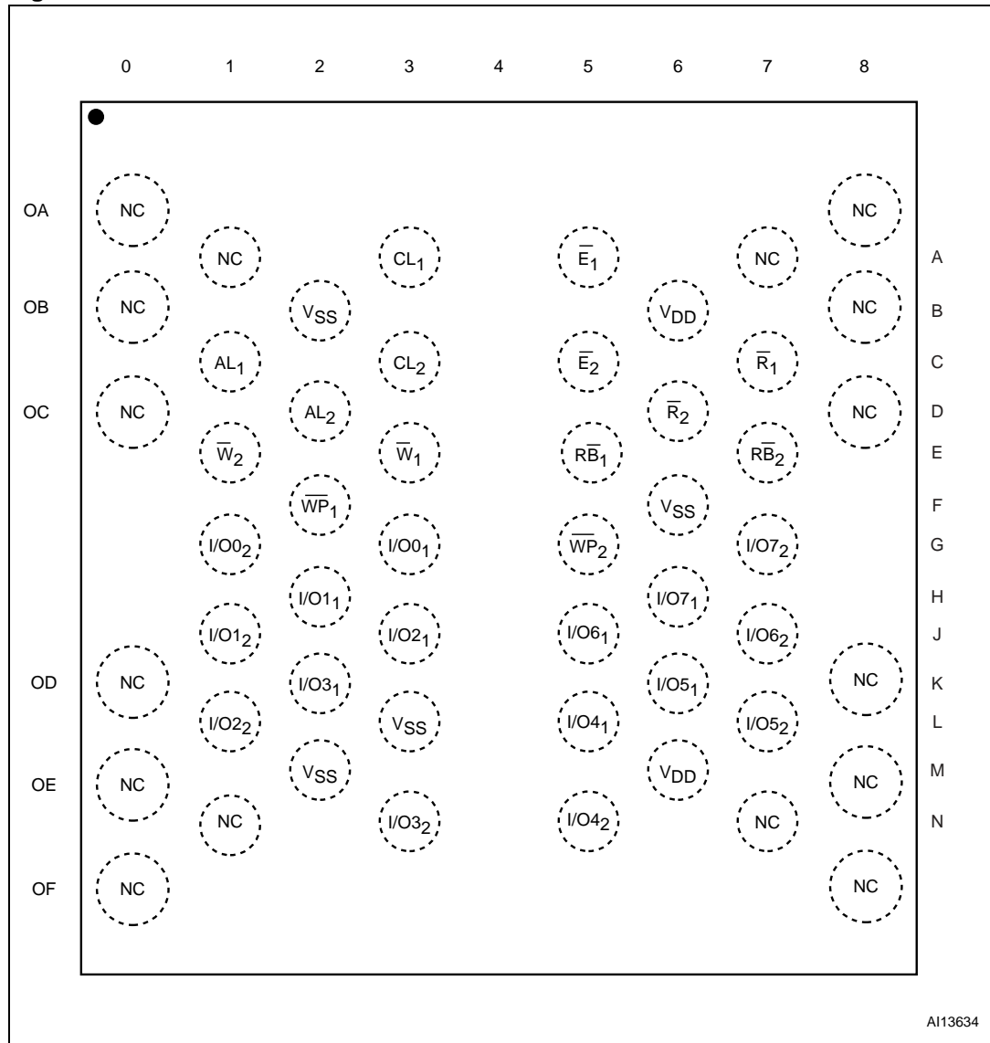
Figure 5. LGA52 connections for the NAND08G-B4C devices
