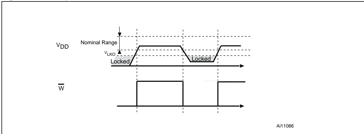
Figure 44. Data protection
