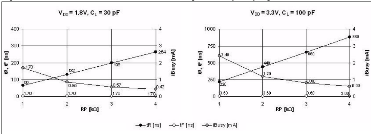
Figure 43. Resistor value versus waveform timings for ready/busy signal
