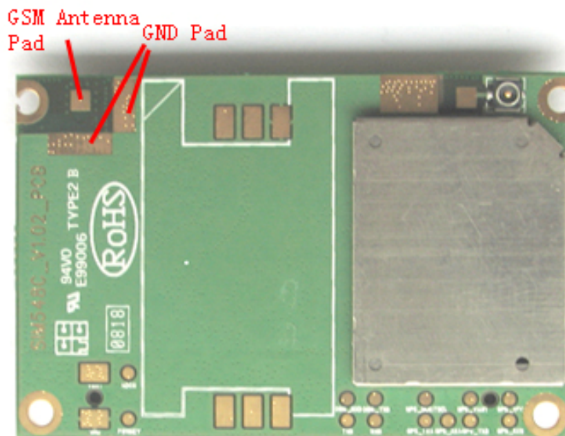
Figure 37: RF connector and RF pad
