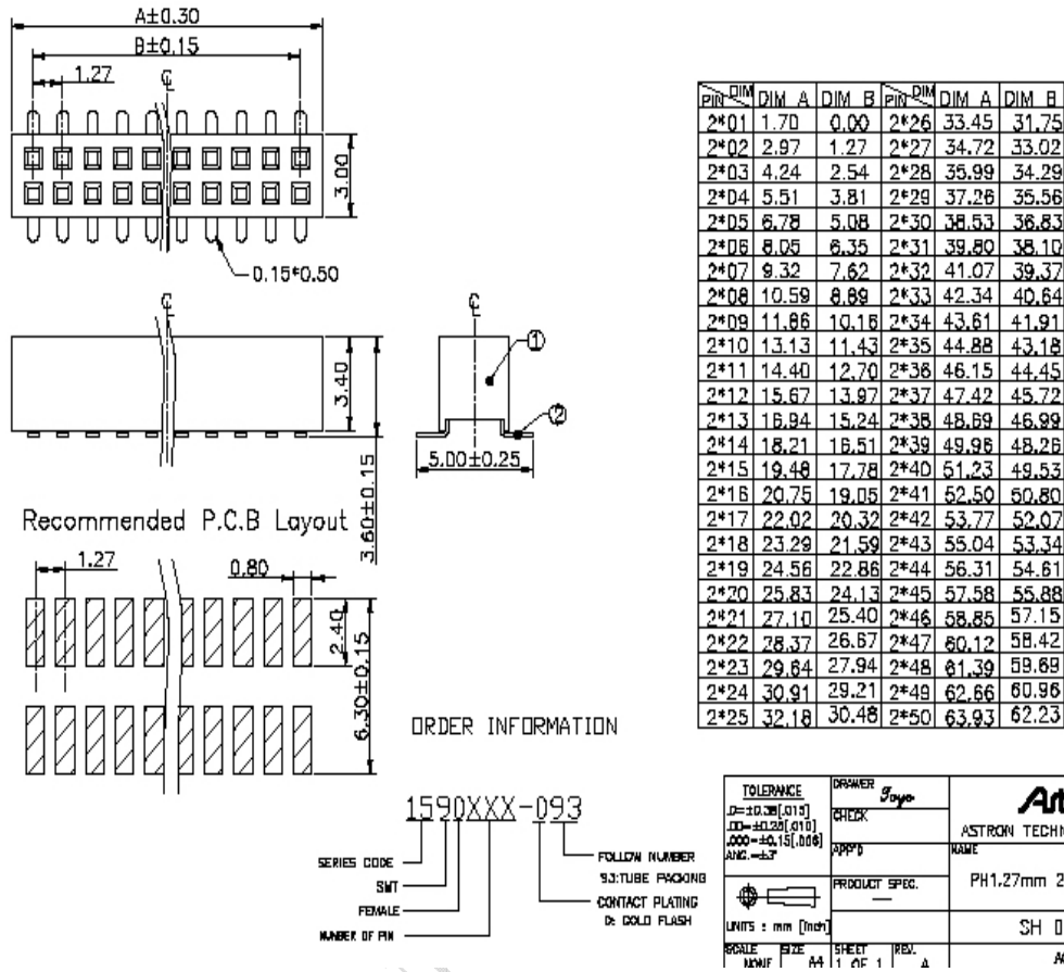
Figure 45: ASTRON1590060-09T-R Board to Board connector
