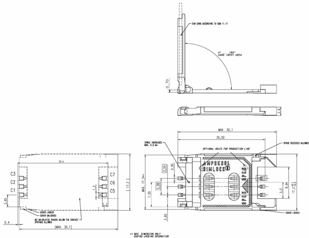
Figure 27: Amphenol C707-10M006 512 2 SIM card holder
