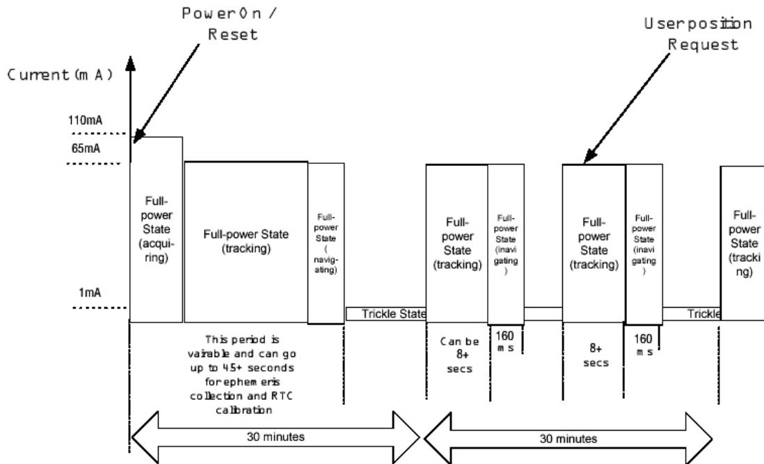
Figure 41: Power consumption in the PTF mode
