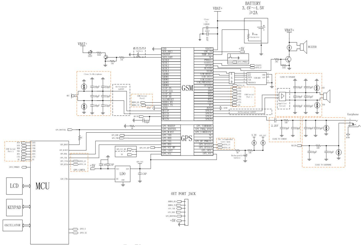
Figure 50: Reference Circuit with external MCU (standalone application for example)
