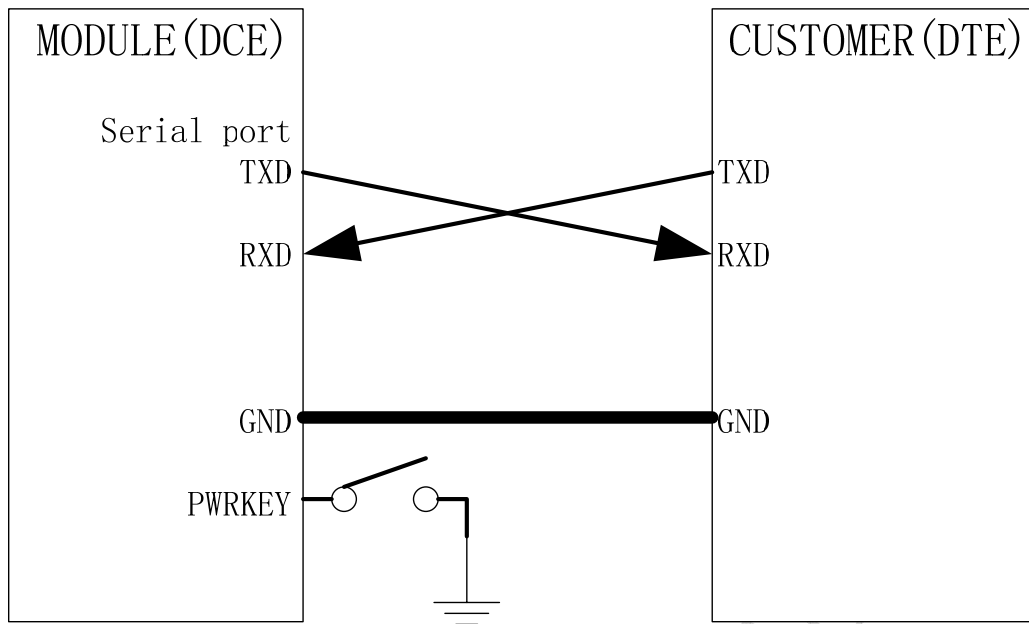
Figure 18: Connection of software upgrade
