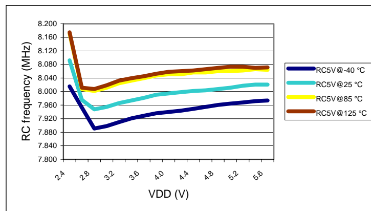
Figure 63. Frequency vs voltage at four different ambient temperatures (RC at 5 V)
