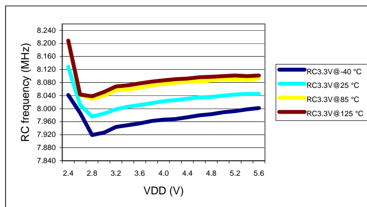
Figure 64. Frequency vs voltage at four different ambient temperatures (RC at 3.3 V)
