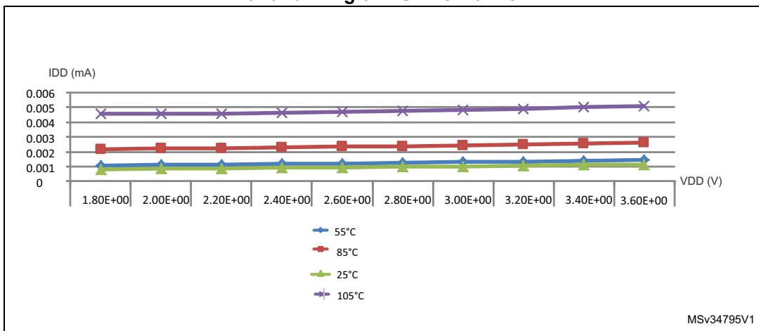
Figure 16. I DD vs V DD , at T A = 25/55/85/105 °C, Stop mode with RTC disabled, all clocks off
