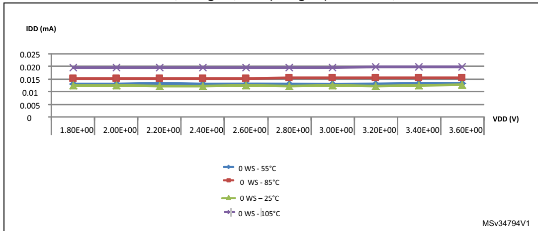
Figure 14. I_{DD} vs V_{DD} , at T_A = 25/55/ 85/105 °C, Low-power run mode, code running from RAM, Range 3, MSI (Range 0) at 64 KHz, 0 WS
