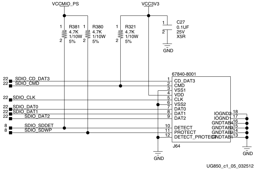
Figure 1-7: SD card interface
