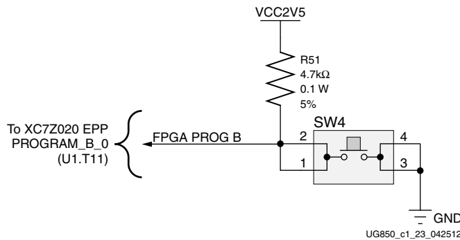
Figure 1-25: PROG_B Pushbutton SW4
