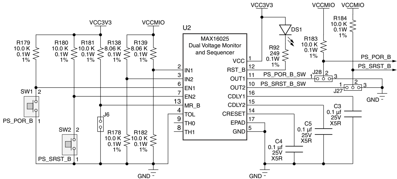
Figure 1-26: PS Power On and System Reset Circuitry
