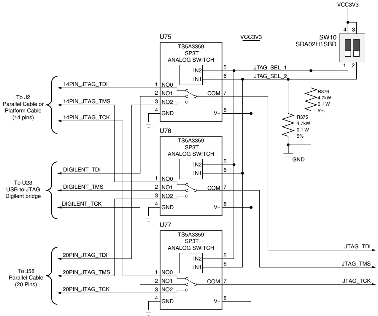
Figure 1-9: PL JTAG Programming Source Analog Switch
