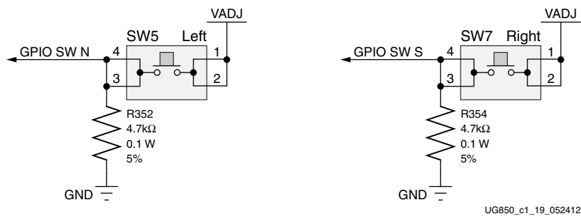
Figure 1-21: User Pushbuttons
