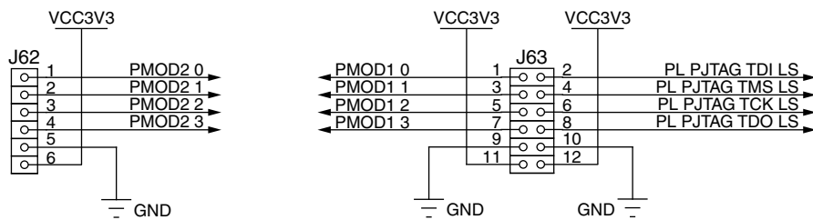
Figure 1-23: User GPIO Headers
