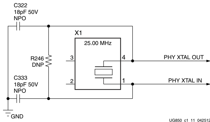
Figure 1-13: Ethernet PHY Clock Source
